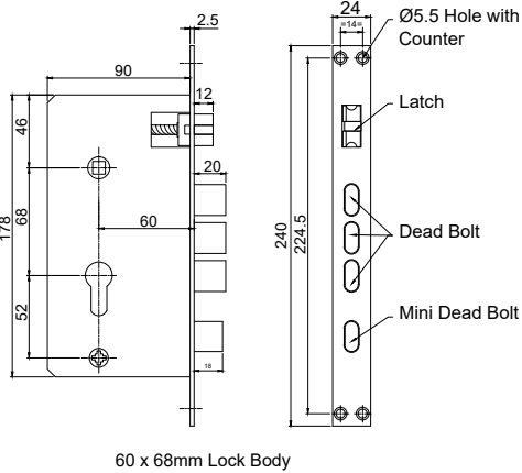
60 x 68mm Lock Body
