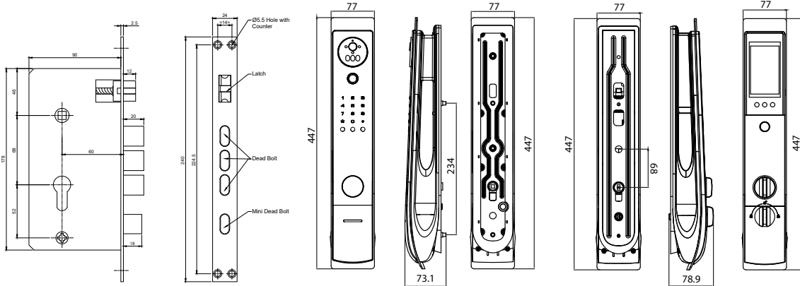
60 x 68mm Lock Body
