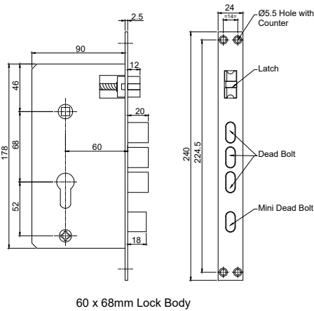
60 x 68mm Lock Body
