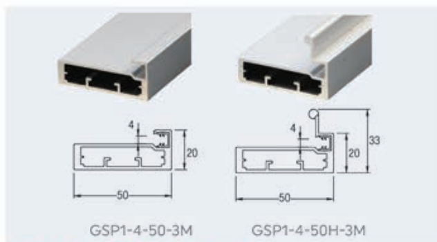
Aluminium Profile Glass Shutter 50mm
