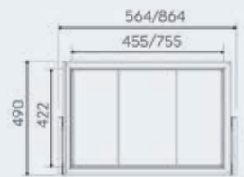
Wardrobe Pull out 2 Shoe Rack - Soft Close
