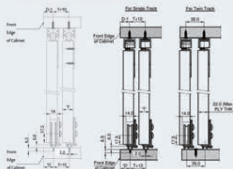
Hi Slide 90 (Demo Track)
