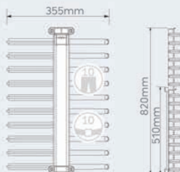
Wardrobe Pull out Hanger - Trouser/Saree Double Cabinet Width: 750mm
