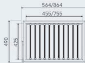
Wardrobe Pull out 2 Drawer Organiser (Soft Close)
