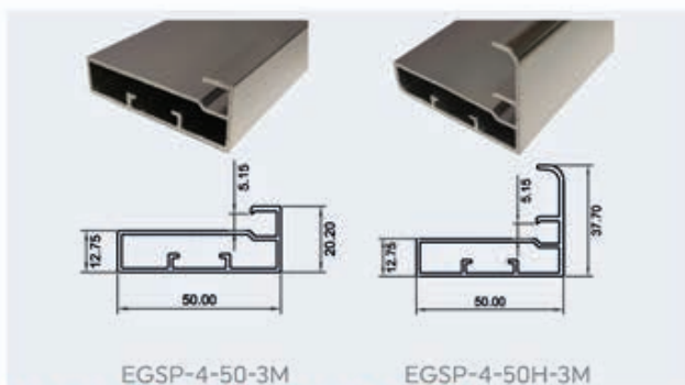
Aluminium Profile Glass Shutter Euro 50mm
