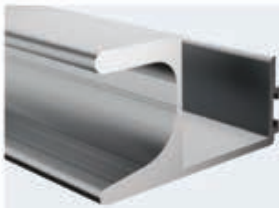
19/25 mm Wardrobe Edge Profile with Inset Handle 2
