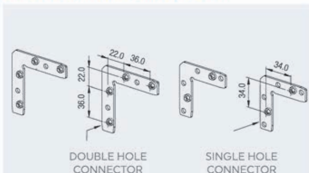
Corner Brackets for Glass Shutter Profile
