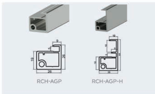
Aluminium Profile For Recessed Hinges.
