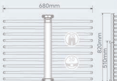
Wardrobe Pull out Hanger - Trouser/Saree Double Cabinet Width: 750mm
